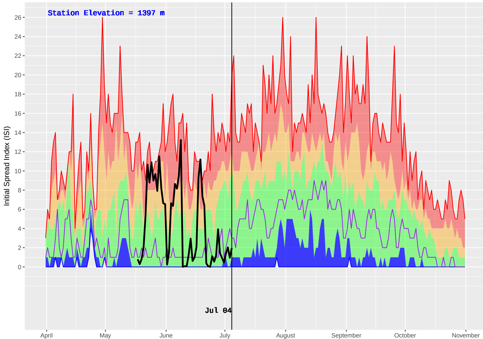
NANCY GREEN (407) : Historical (1992–2016) and Current (2018) Noon Initial Spread Index (ISI)
