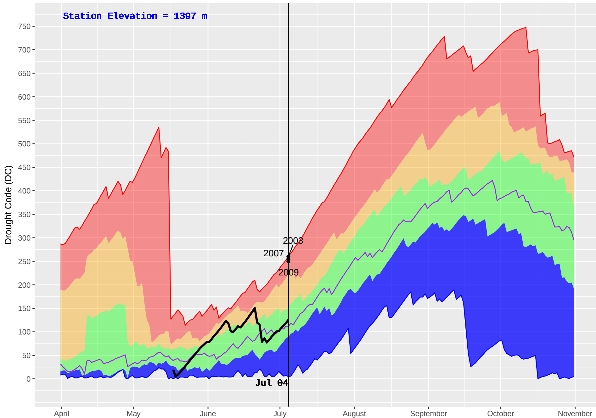
NANCY GREEN (407) : Historical (1992–2016) and Current (2018) Noon Drought Code (DC)
